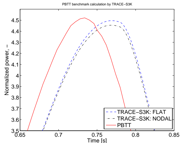
Figure 9. Relative power for different coupling options
