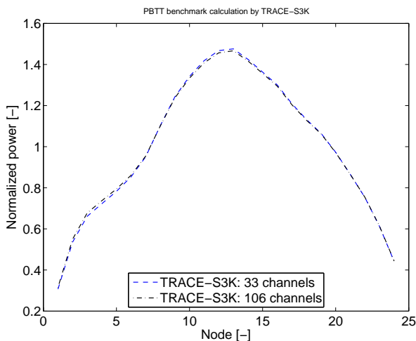
Figure 10. Initial core axial power profile for 33- and 106-channels models
