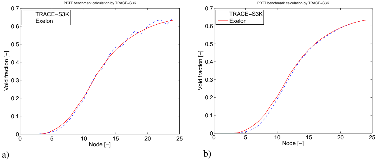
Figure 2. Initial core void profile: a) K-loss factors according to the specifications, b) K-loss distributed uniformly along the channels
