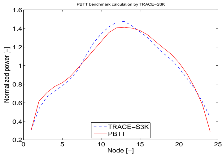
Figure 3. Initial core axial power profile
