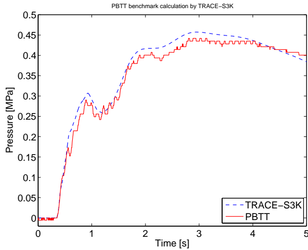
Figure 4. Dome pressure change
