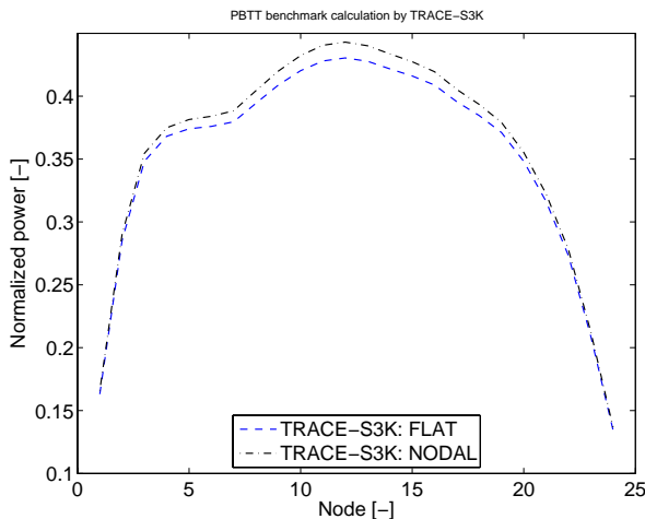
Figure 8. Initial axial power profile for selected fuel assembly
