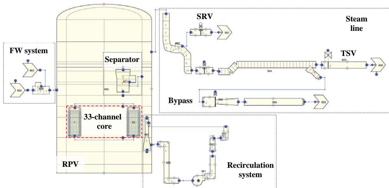
Figure 1. Schematic TRACE model for PB2 TT2
