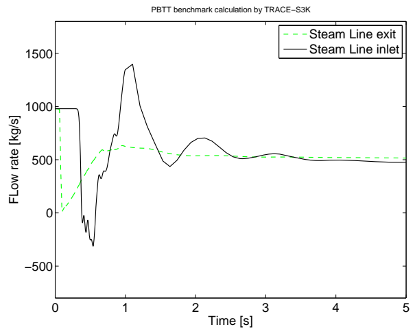
Figure 7. Steam line flow rate
