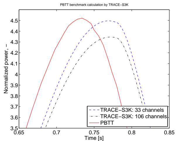
Figure 11. Relative power for 33- and 106-channels models
