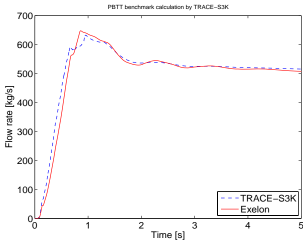
Figure 6. Turbine bypass valve flow rate
