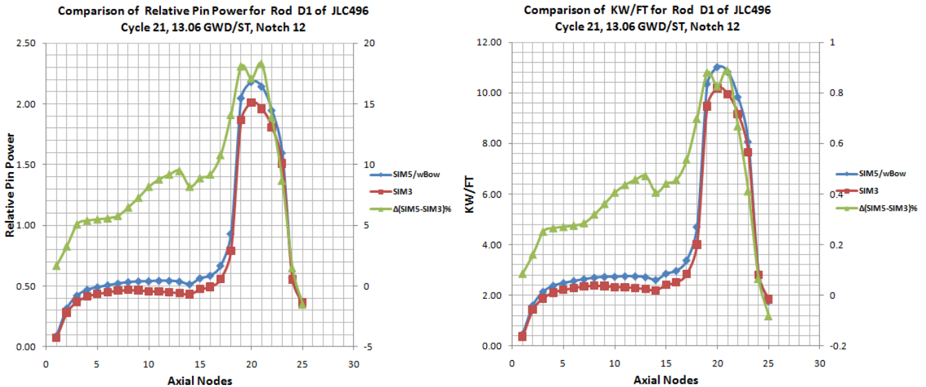
Fig. 9. Relative pin power and KW/FT (SIM5 with QTH & BOW vs. SIM3) for rod D1 of JLC496, C21 at 13.06 GWD/ST
