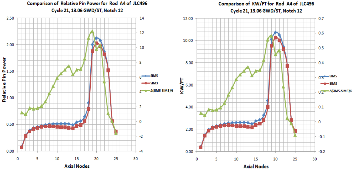
Fig. 5. Relative pin power and KW/FT (SIM5 with QTH vs. SIM3) for rod A4 of JLC496, C21 at 13.06 GWD/ST
