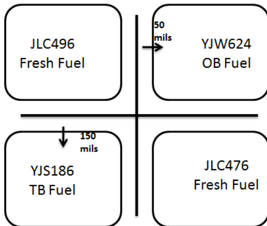
Fig. 3. Control cell with an assumed channel bow
