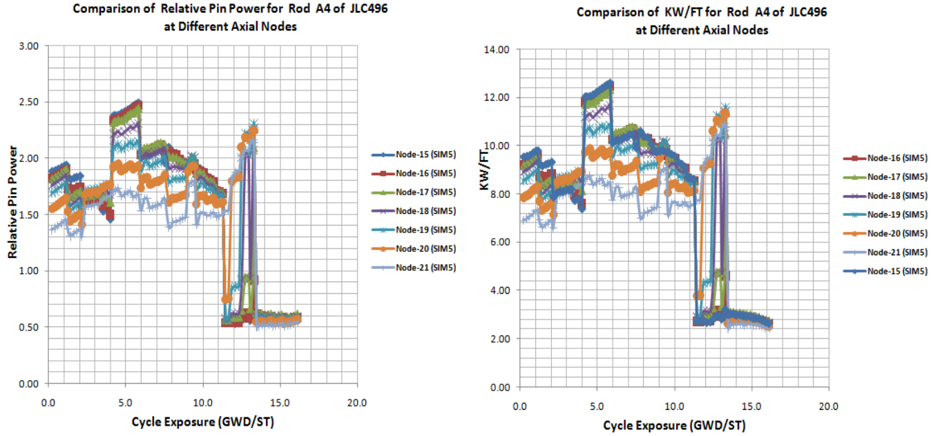
Fig. 10. SIMULATE5 calculated relative pin power and KW/FT for rod A4 of JLC496 at several axial nodes
