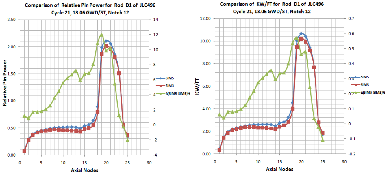
Fig. 6. Relative pin power and KW/FT (SIM5 with QTH vs. SIM3) for rod D1 of JLC496, C21 at 13.06 GWD/ST
