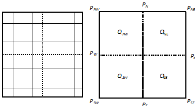
Fig. 1. SIMULATE5 Submeshes and quarter-assemblies model
