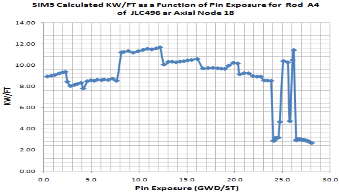
Fig. 11. SIMULATE5 calculated KW/FT for rod A4 of JLC496 at node 18
