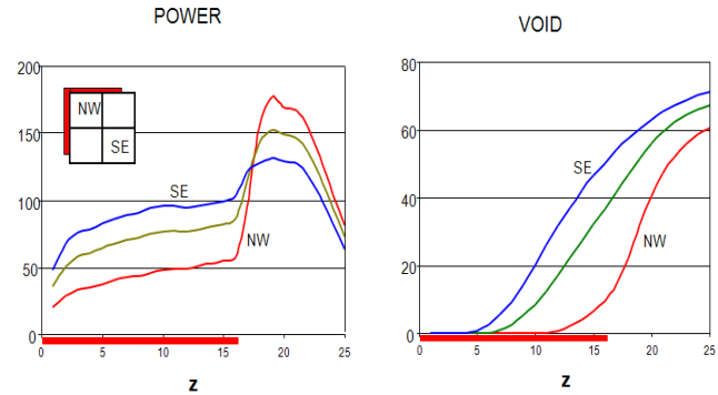
Fig. 2. SIMULATE5 power & void distribution with QTH option
