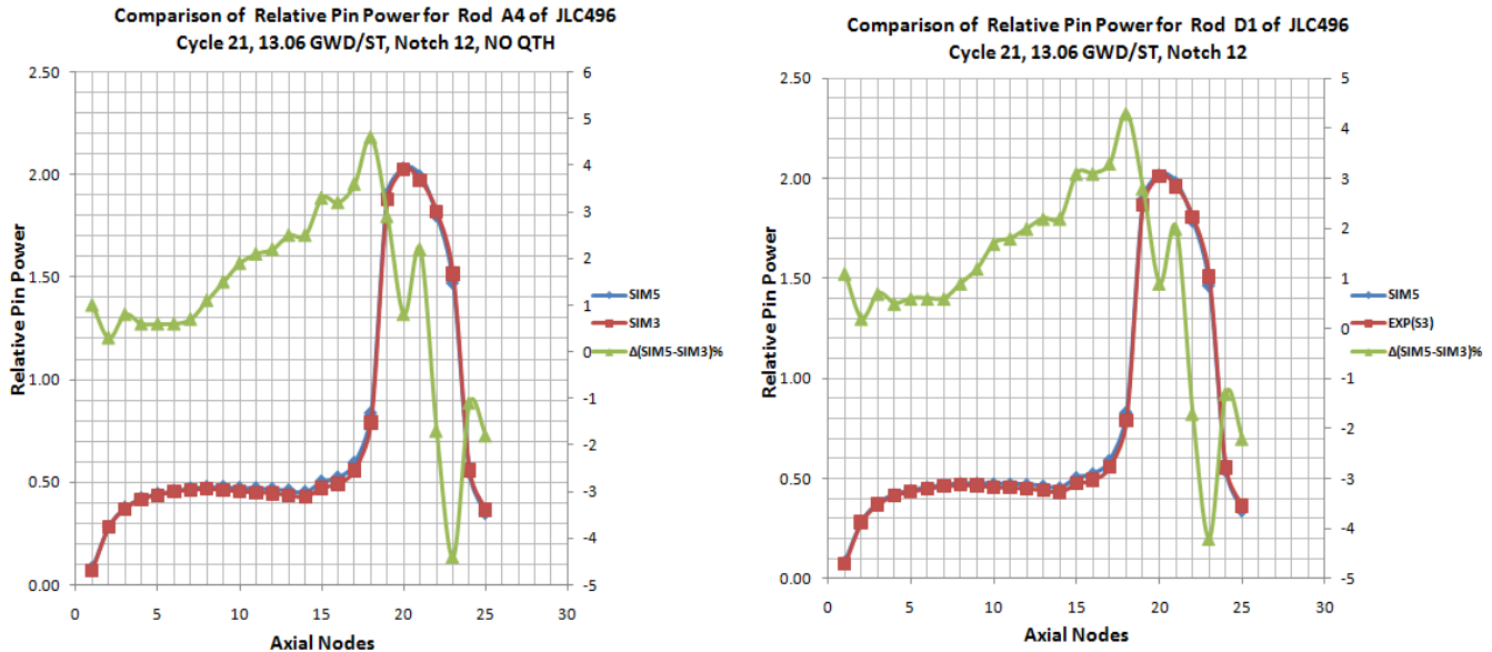
Fig. 7. Relative pin power (SIM5 without QTH vs. SIM3) for rods A4 & D1 of JLC496, C21 at 13.06 GWD/ST
