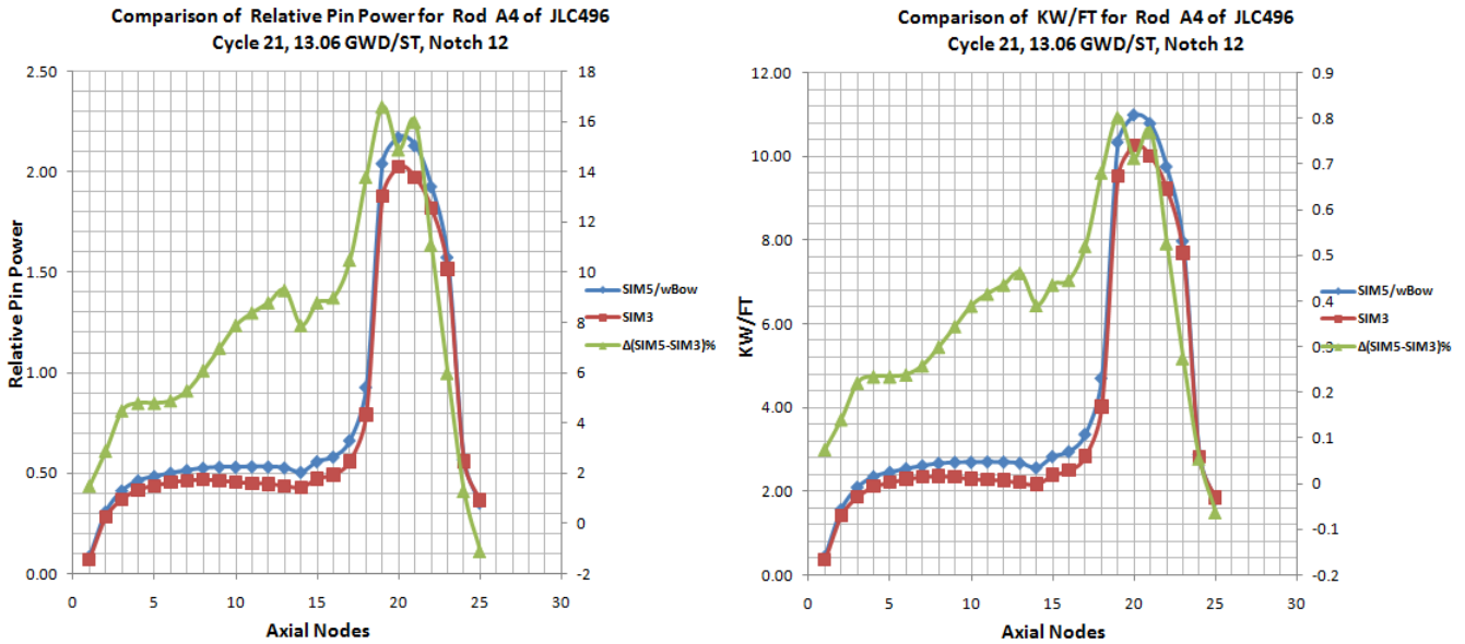
Fig. 8. Relative pin power and KW/FT (SIM5 with QTH & BOW vs. SIM3) for rod A4 of JLC496, C21 at 13.06 GWD/ST
