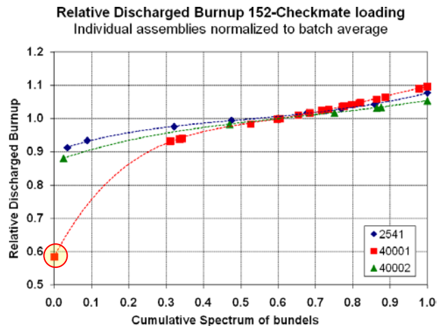
Fig. 14. Skewness and Spread in Discharged Burnup 152 ACCD Equilibrium Core
