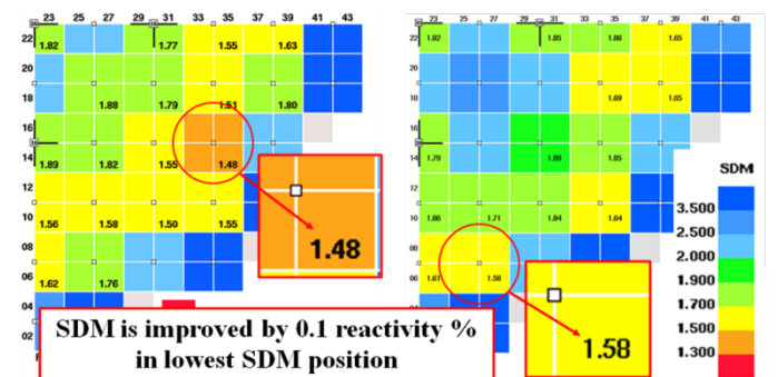
Fig. 4. Shutdown Margin Comparison
