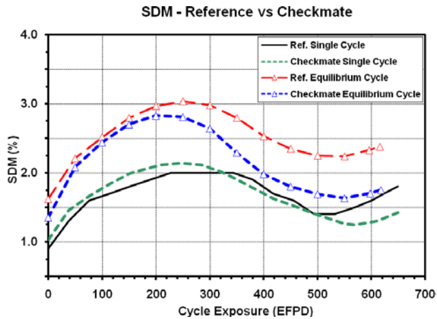
Fig. 8. Shut Down Margin Comparisons
