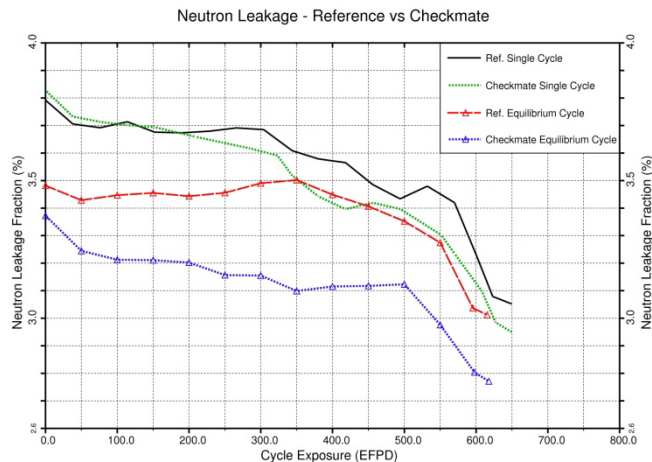
Fig. 9. Neutron leakage Comparisons
