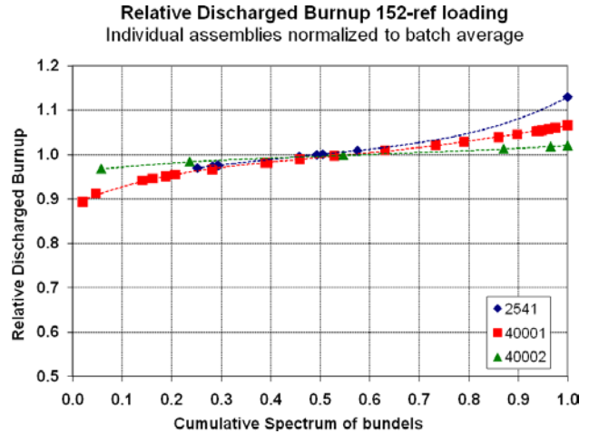
Fig. 13. Skewness and Spread in Discharged Burnup 152 Reference Equilibrium Core
