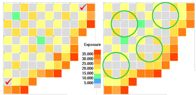
Fig. 1 Checkerboard vs ACCD Loading - 152 Fresh
