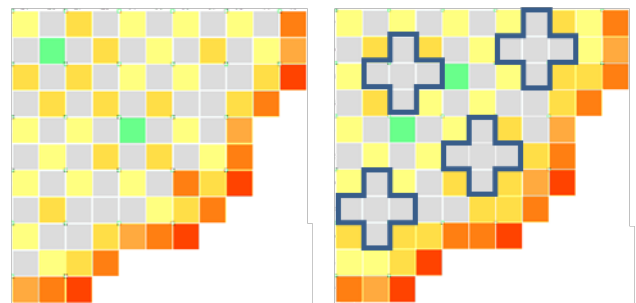
Fig. 10. Single Cycle, 160 Fresh Loading Reference vs. ACCD
