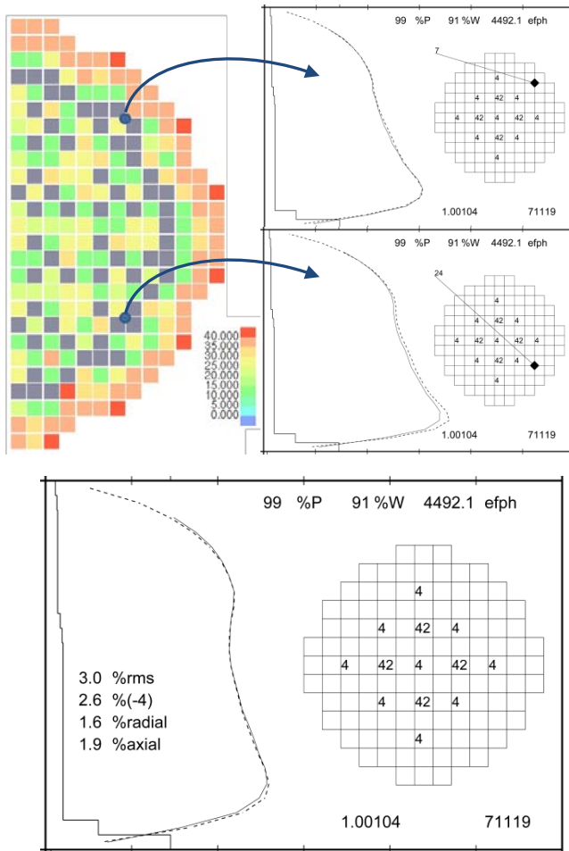
Fig. 15. TIP RMS face adjacent core loading
