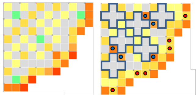
Fig. 11. Equilibrium Cycle, 160 Fresh Loading Reference vs. ACCD
