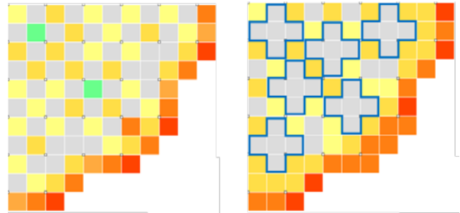
Fig. 6. Equilibrium Cycle, 152 Fresh Loading Reference vs. ACCD
