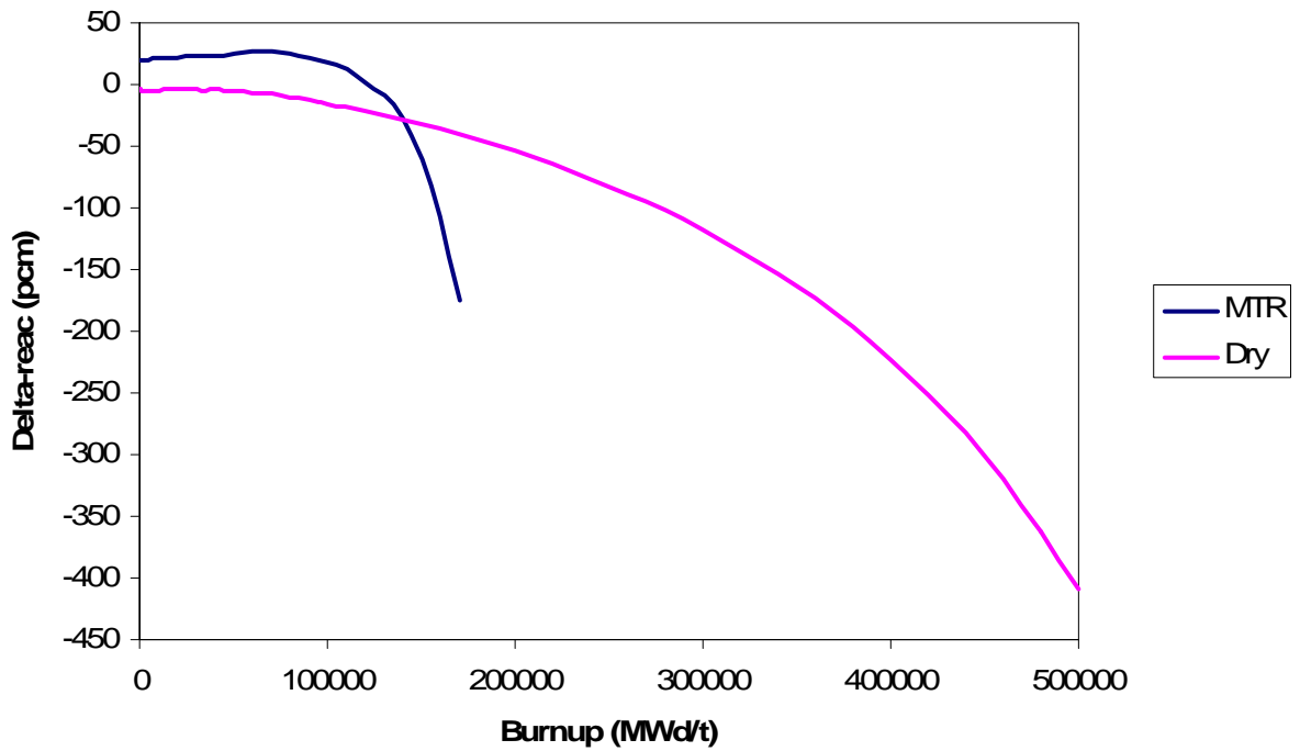
Figure 4. Results of test matrix MTR assembly and Dry MOX pin-cell calculations, comparing MOC to CP.
