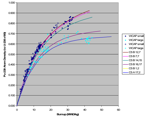
Figure 6. Yankee Rowe ^{239}\text{Pu} concentration relative to initial ^{238}\text{U} concentration.
