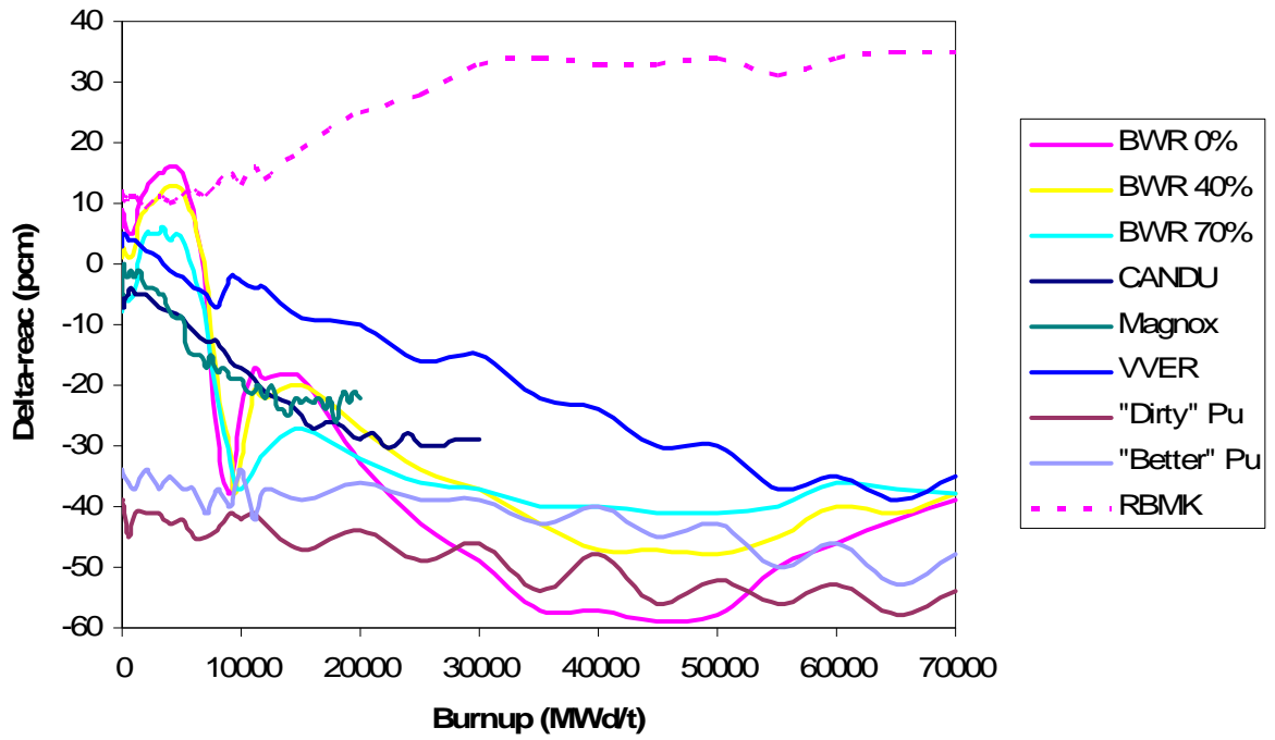
Figure 3. Results of test matrix calculations, comparing MOC to CP.
