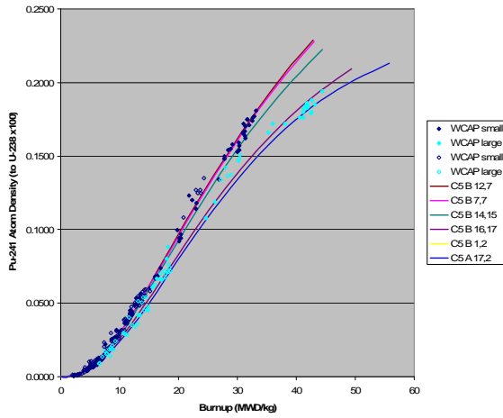
Figure 7. Yankee Rowe ^{241}\text{Pu} concentration relative to initial ^{238}\text{U} concentration.
