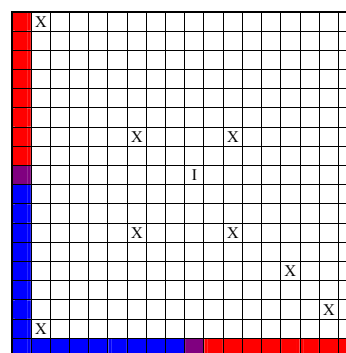
Figure 2. Locations of pins sampled in Yankee Rowe assembly (X), with control blade locations shown for Type A (blue) and Type B (red) assemblies.
