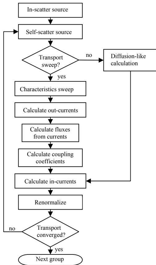
Figure 1. The calculation scheme for the MOC transport solver in HELIOS-2.
