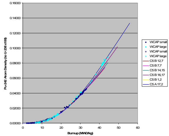
Figure 8. Yankee Rowe ^{242}\text{Pu} concentration relative to initial ^{238}\text{U} concentration.
