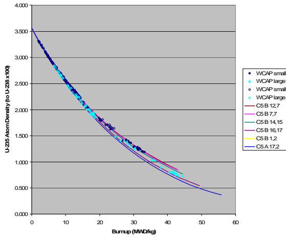
Figure 5. Yankee Rowe ^{235}\text{U} concentration relative to initial ^{238}\text{U} concentration.
