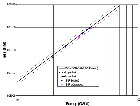
Fig. 3. SNF vs. Würz neutron emission correlation for CLAB BWR assemblies.
