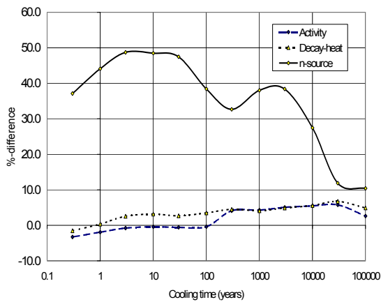
Fig. 1 %-difference in activity, decay heat and neutron source between 3-D and 0-D SNF calculations (BWR fuel at 41 GWd/t).
