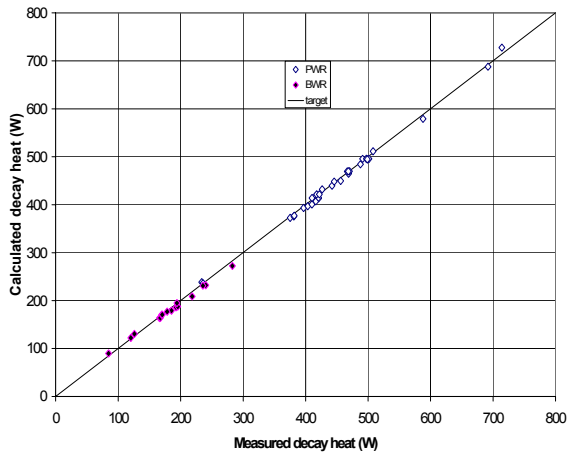
Fig. 2 SNF calculated versus measured decay heat of 49 BWR and PWR spent fuel assemblies
