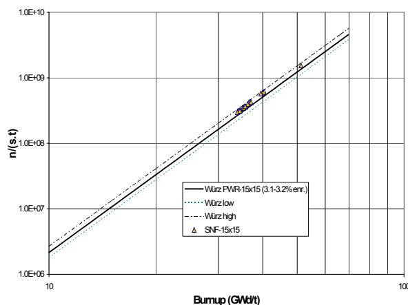
Fig. 4. SNF vs. Würz neutron emission correlation for CLAB PWR fuel assemblies.
