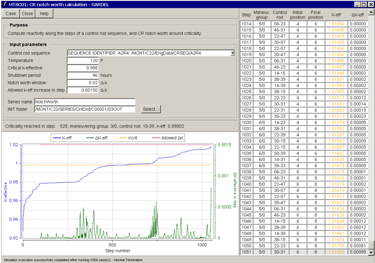
Figure 5 Notch worth calculation interface
