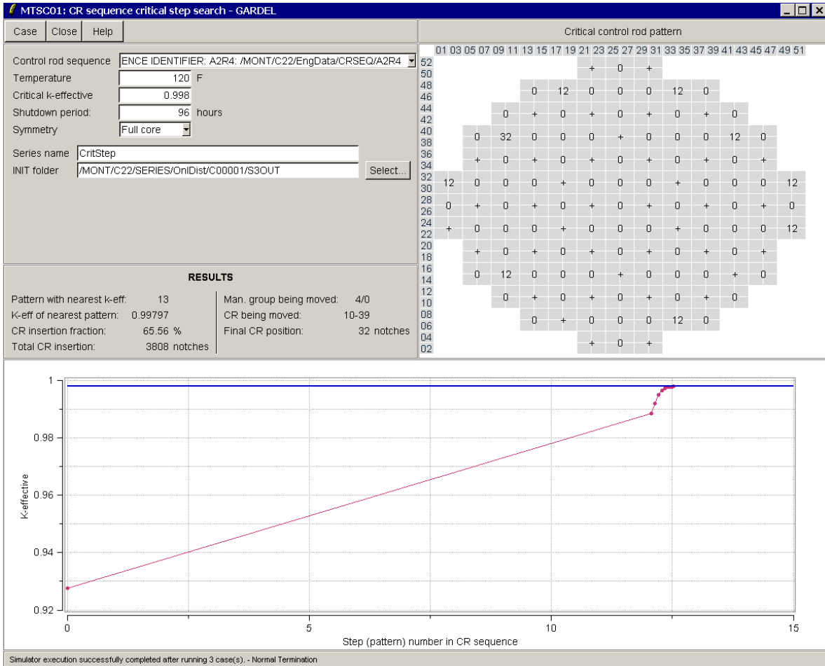
Figure 4 Estimated Critical Position interface
