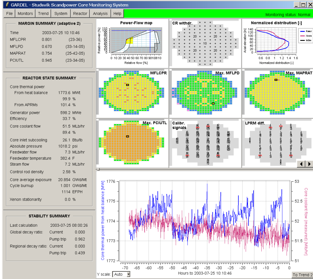
Figure 2 Main GARDEL-BWR Graphical interface.
