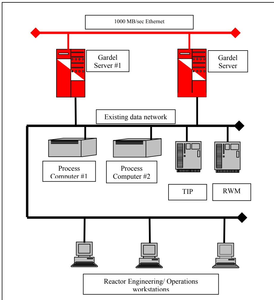
Figure 1 GARDEL-BWR system hardware configuration
